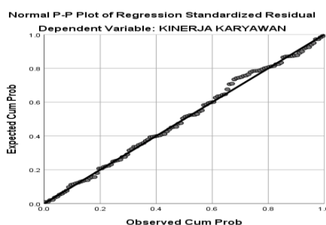
Figure 2. Normality Test
