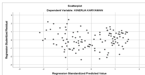
Figure 3. Heteroscedasticity Test
